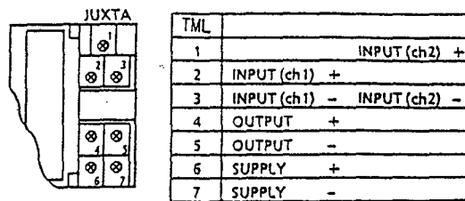
Fig.9 Wiring Diagram
